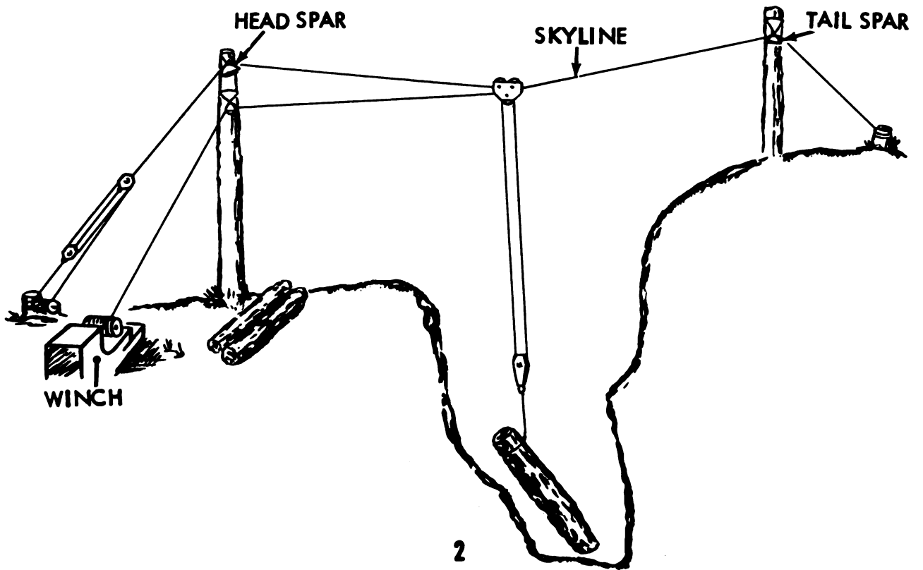
LOGGING A BOX CANYON WITH A SKYLINE
